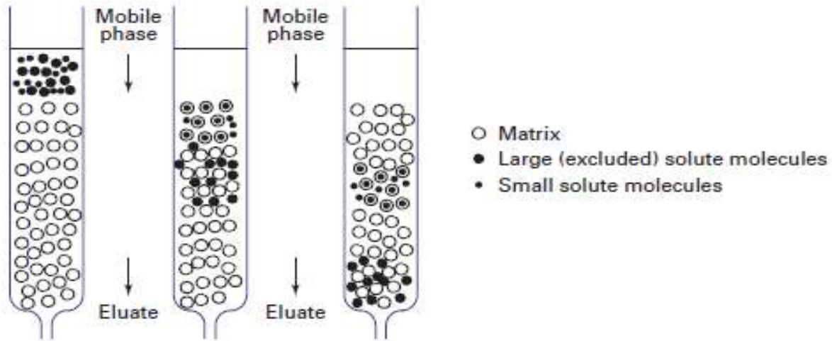
Fig. 11.14. Separation of different size molecules by exclusion chromatography. Large (excluded) molecules are eluted first in the void volume.
