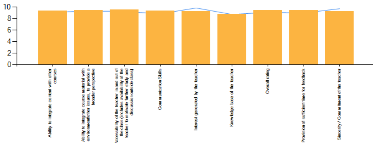
Figure4:SplineDiagram-scoreacrosscourse
